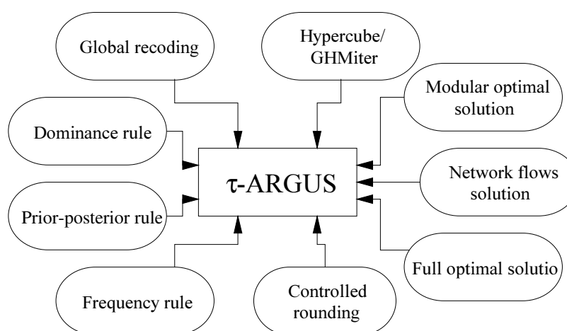
Figure 4-1: Overview of the \tau -ARGUS architecture
