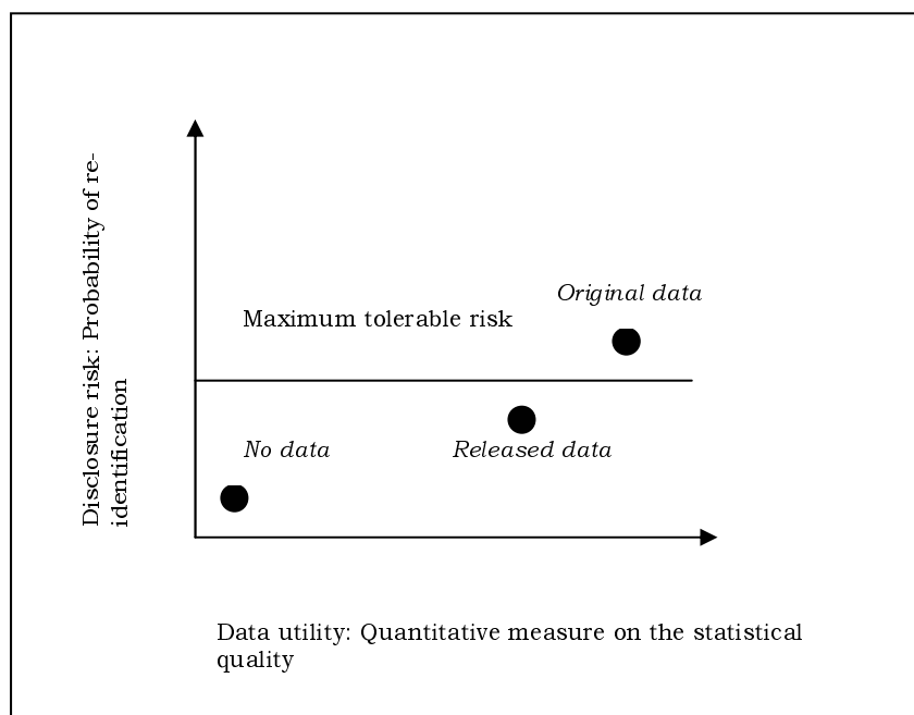
Figure 1-1: R-U Confidentiality map
