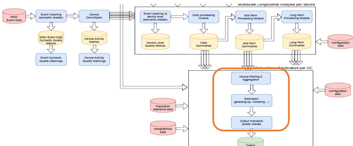
Figure 6: Representation Multi-MNO data fusion and the MNO-to-NSI data transfer in the basic approach for multi-MNO data fusion
