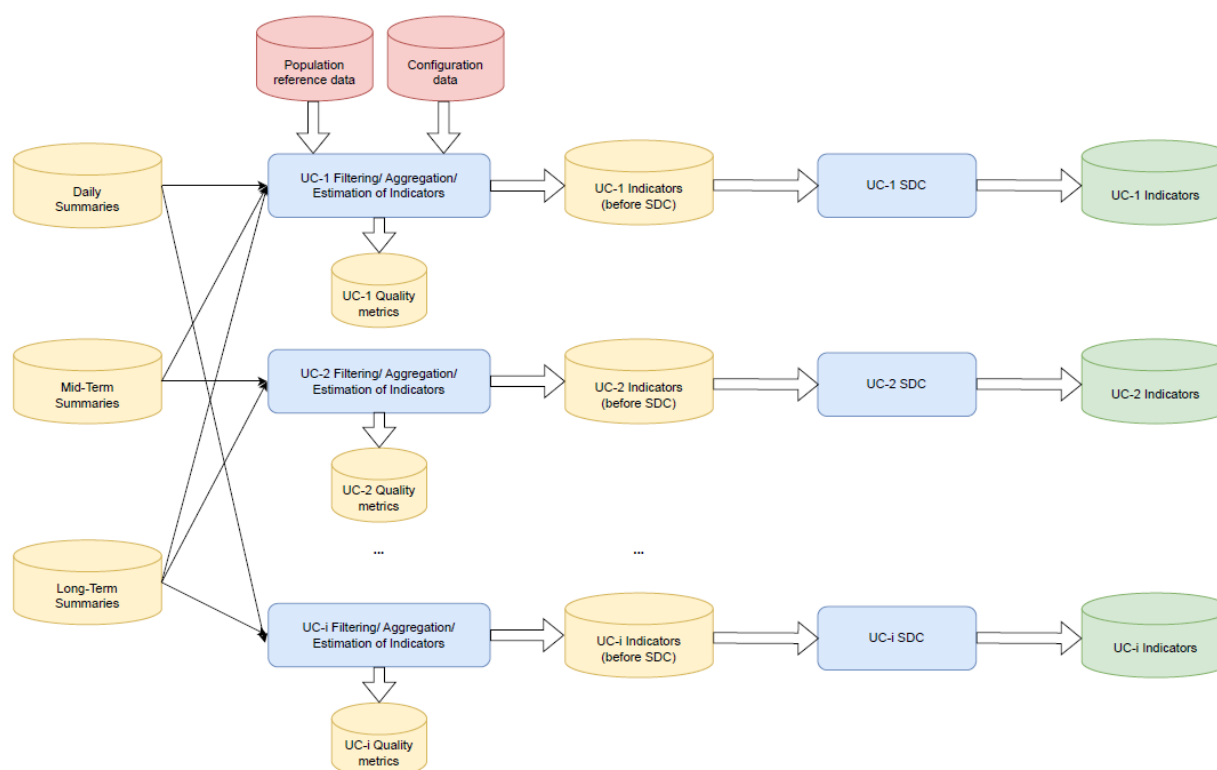
Figure 5: Representation of the integration and aggregation process
